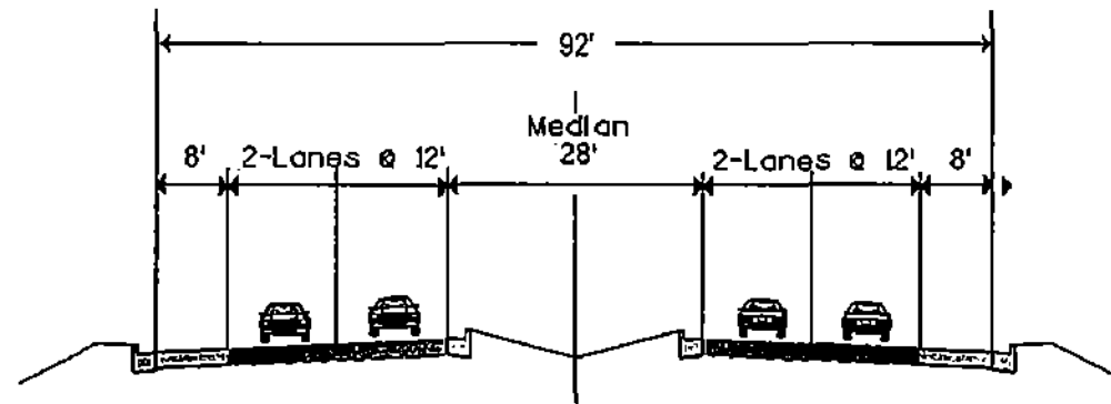
Existing Typical Section (Total R/W Varies from 115' to 170')
