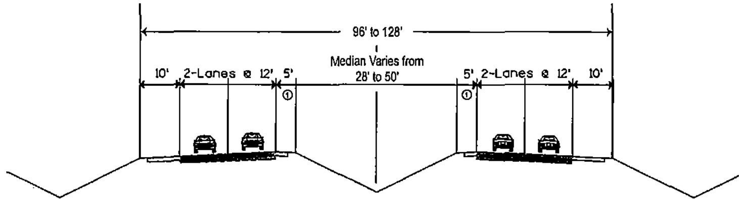
Existing Typical Section (Total RW Varies from 160' to 235')
