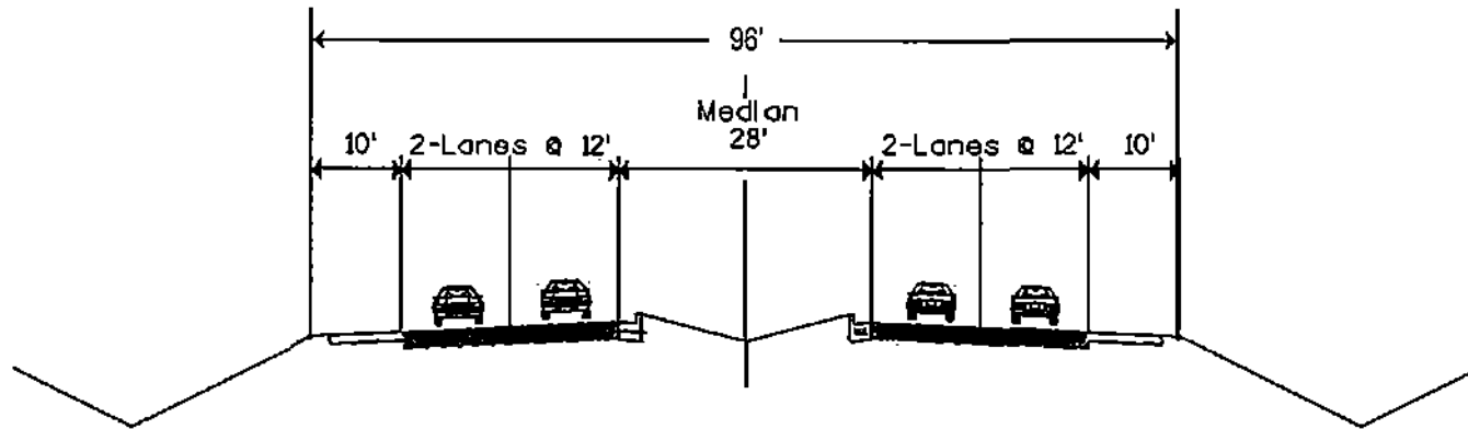
Existing Typical Section (Total R/W Varies from 115' to 170')
