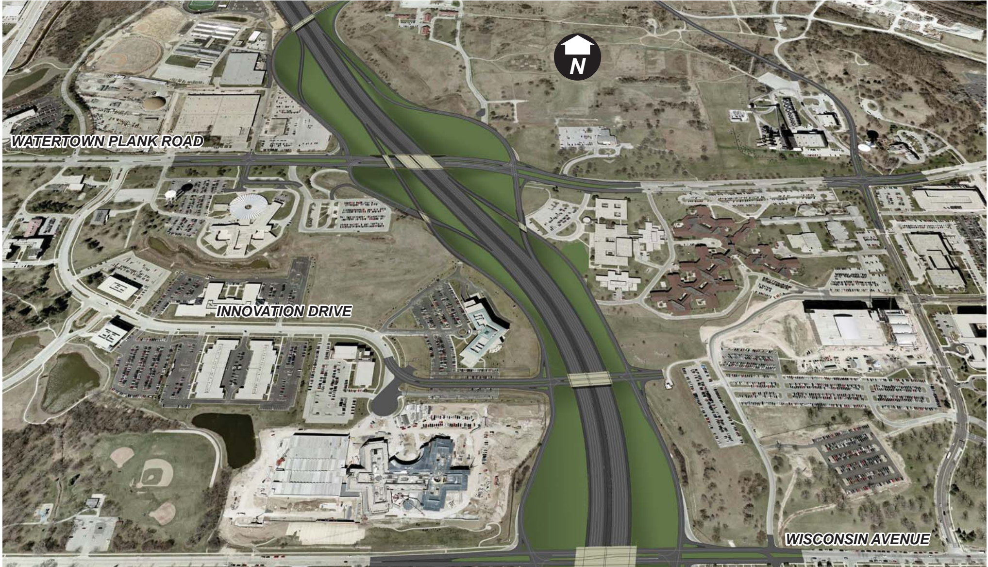
Vista Facing North - M1 Alternative - Wisconsin Ave / Watertown Plank Rd at USH-45
