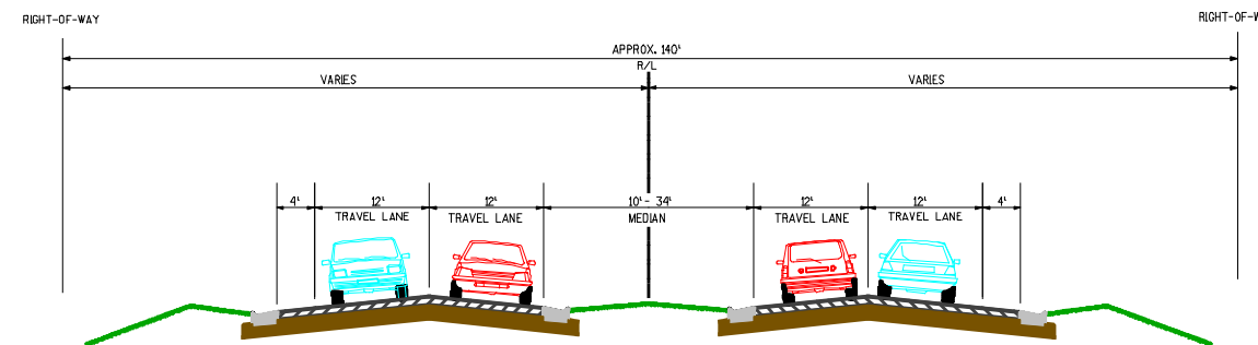
PROPOSED ROUNDABOUT ALTERNATIVE
